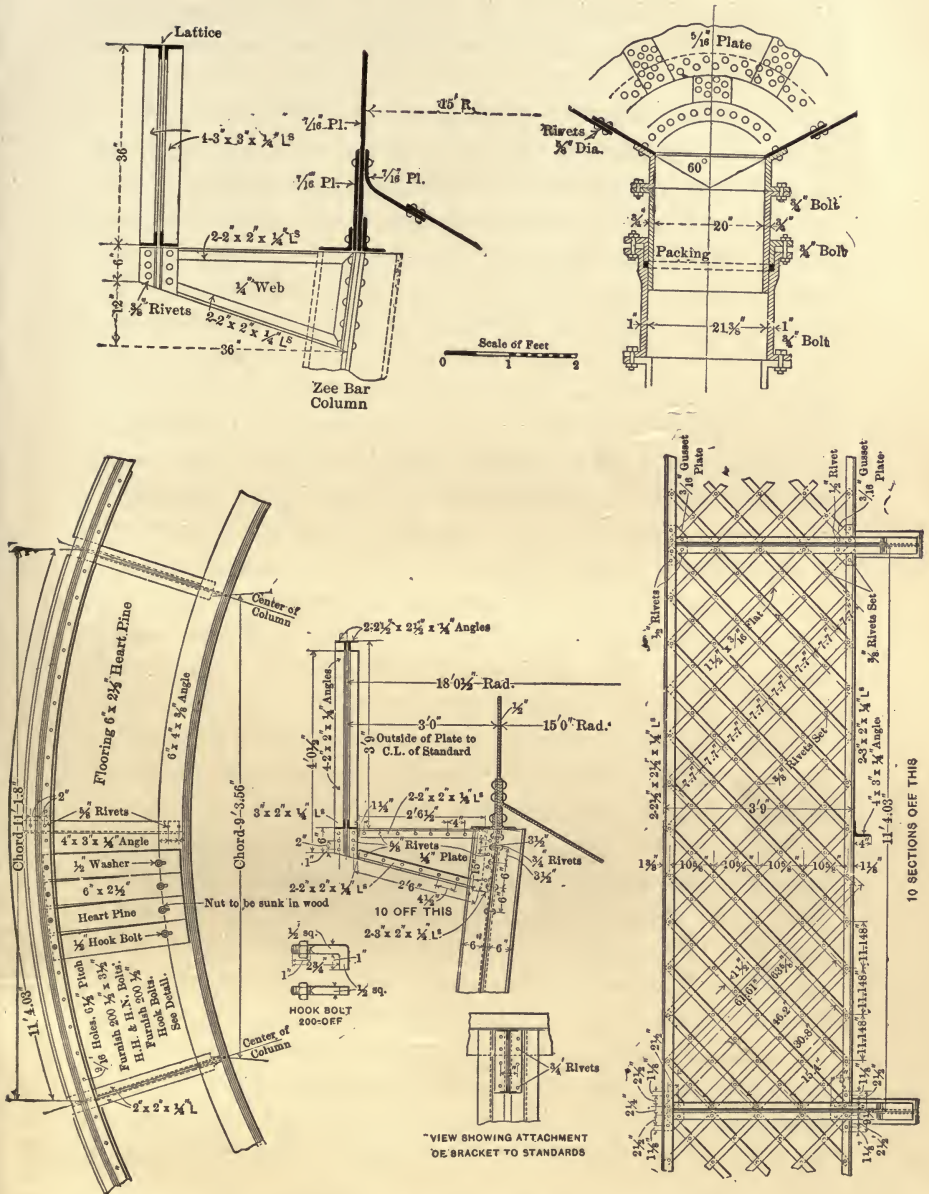
FIG. 1.—TANK DETAILS WATER-TOWER AT JACKSONVILLE, FLA.
